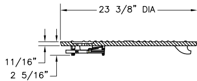
COVER SECTION
