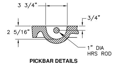
PICKBAR DETAILS
