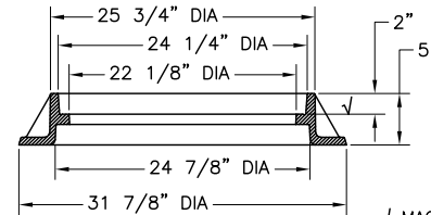
RING SECTION
