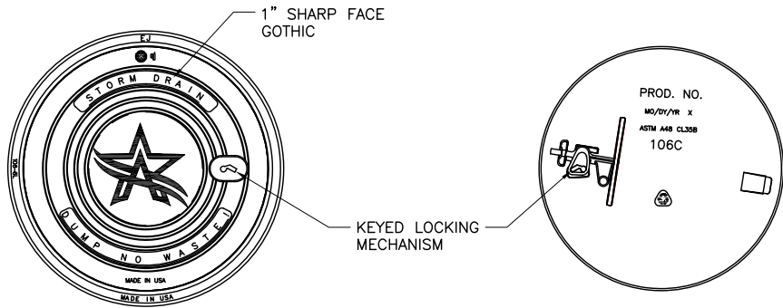
BOTTOM VIEW OF COVER
