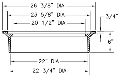
FRAME SECTION
